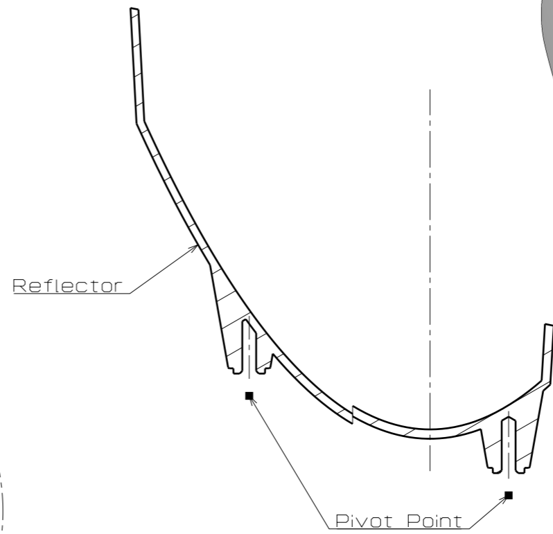
Section Cut A-A
