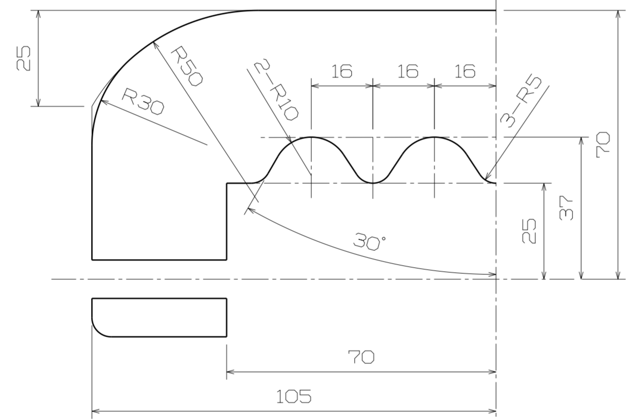
Section Cut B-B CL
