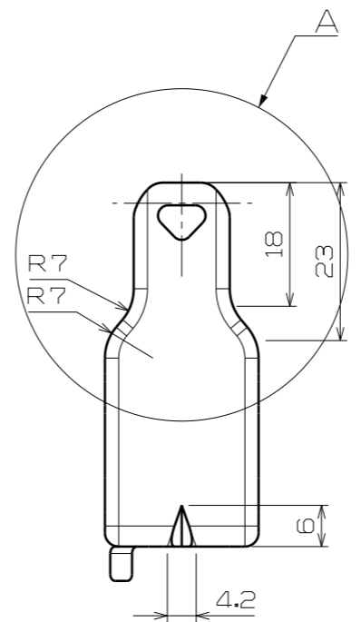
Auxiliary View C
